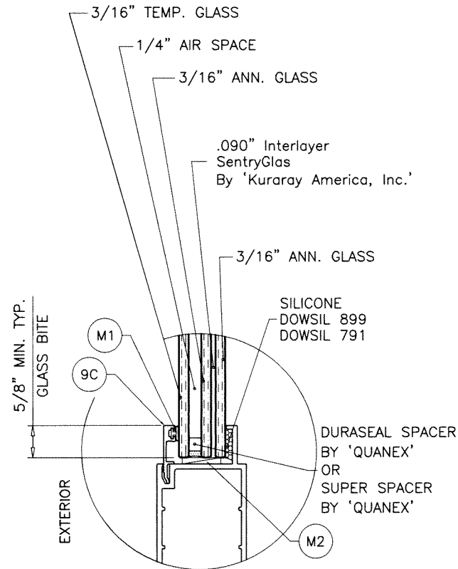
GLASS TYPE 'Ai' 7/8" OVERALL INSUL. LAM. GLASS
