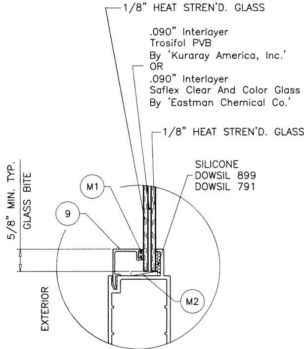
GLASS TYPE 'D' 5/16" OVERALL LAM. GLASS
