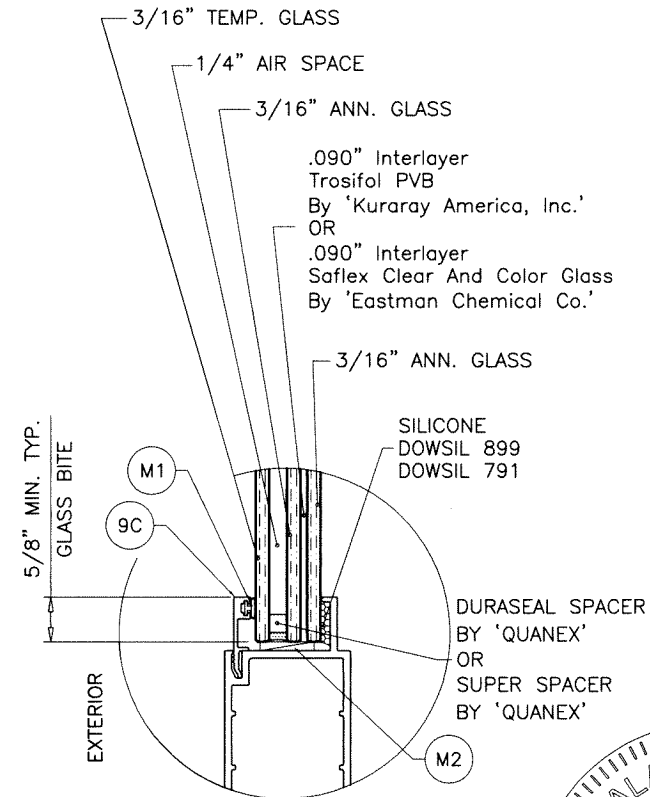
GLASS TYPE 'Fi' 7/8" OVERALL INSUL. LAM. GLASS
