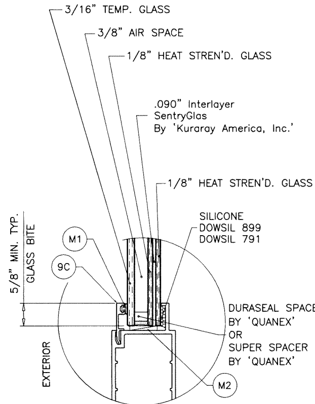
GLASS TYPE 'Ei' 3/4" OVERALL INSUL. LAM. GLASS
