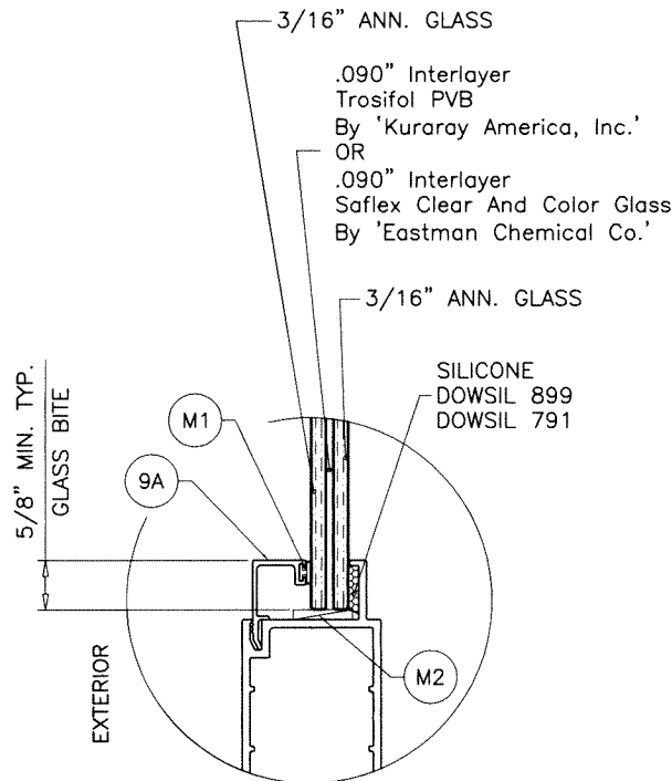
GLASS TYPE 'F' 7/16" OVERALL LAM. GLASS
