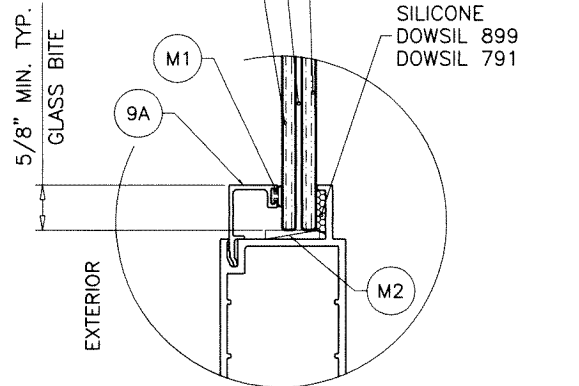
GLASS TYPE 'A' 7/16" OVERALL LAM. GLASS
