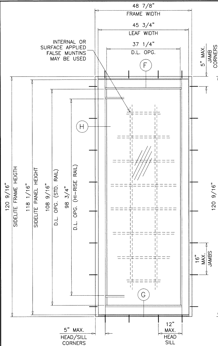
TYPICAL ELEVATION ( O )
