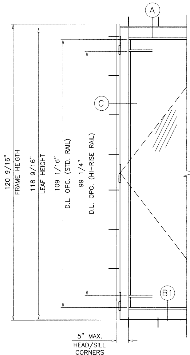
SINGLE OR DOUBLE DOORS WITH ADA SILL
