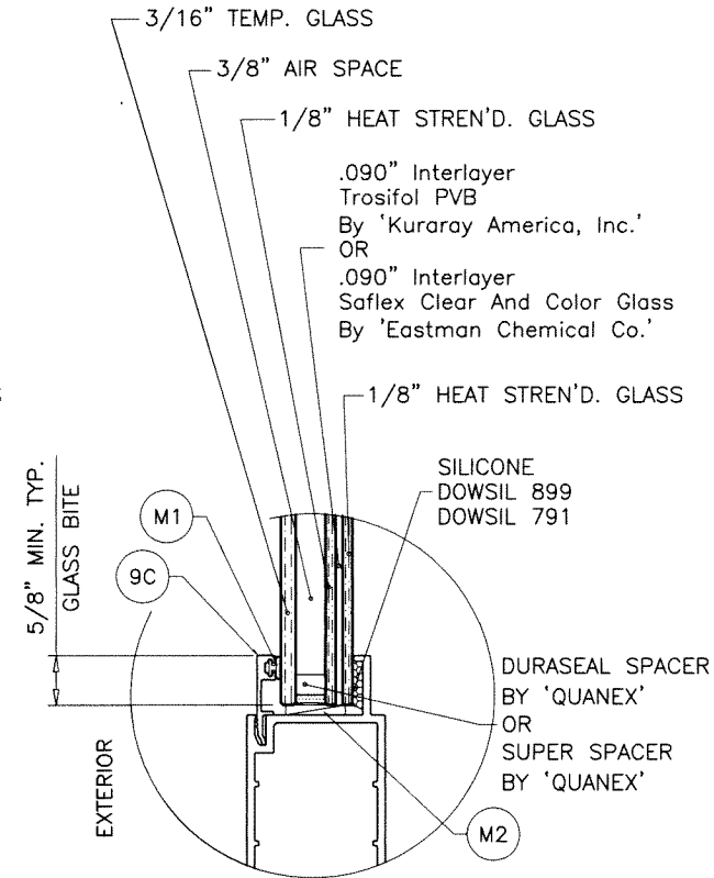
GLASS TYPE 'Di' 7/8" OVERALL INSUL. LAM. GLASS
