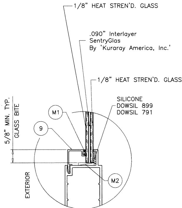
GLASS TYPE 'E' 5/16" OVERALL LAM. GLASS
